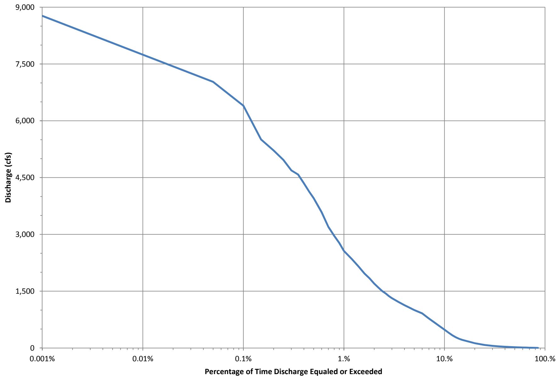
FCP Discharge-Duration Curve - Maple River - 1 - 0.78
