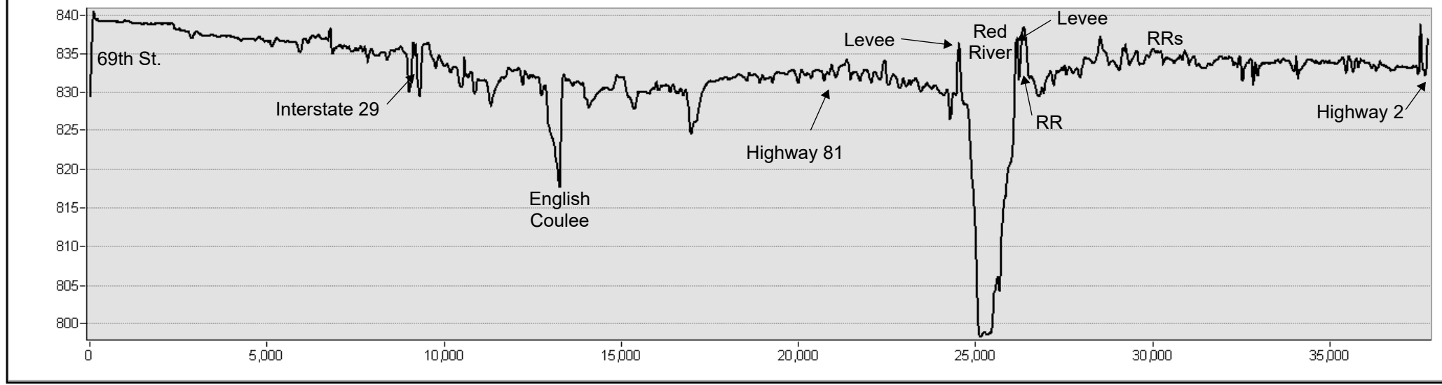
GF 2 Cross Section
