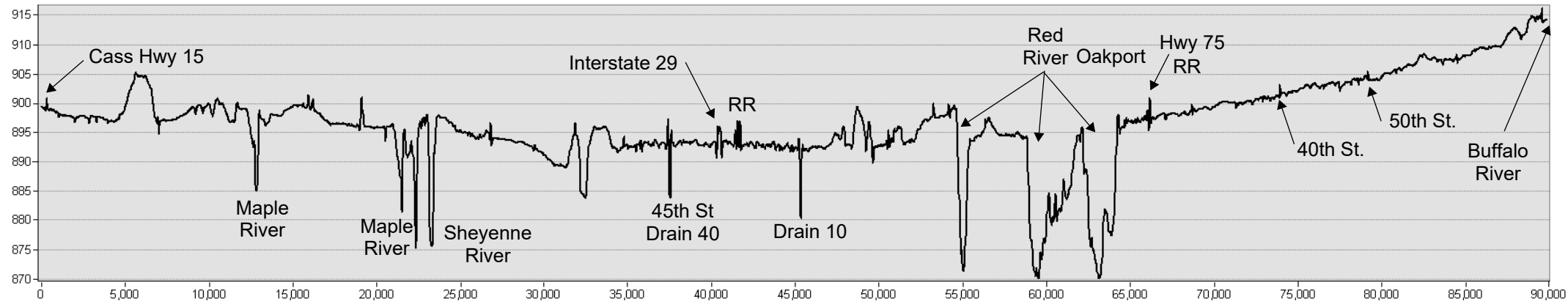
FM 4 Cross Section
