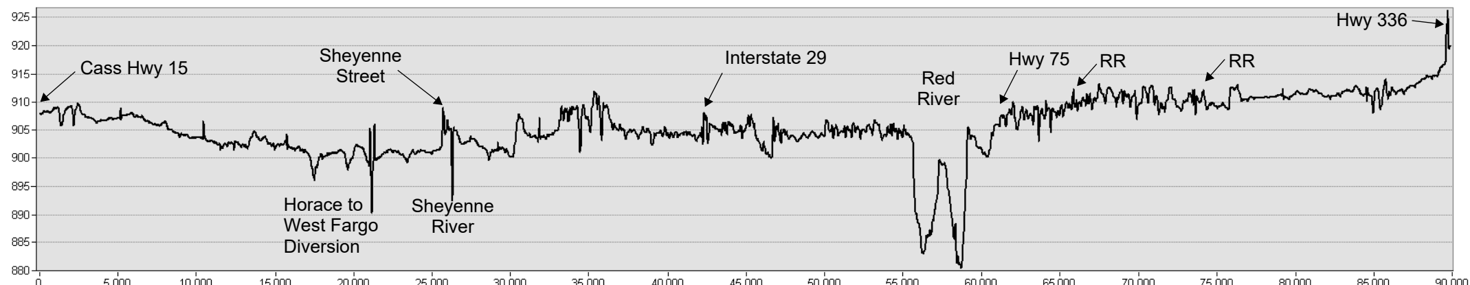
FM 2 Cross Section
