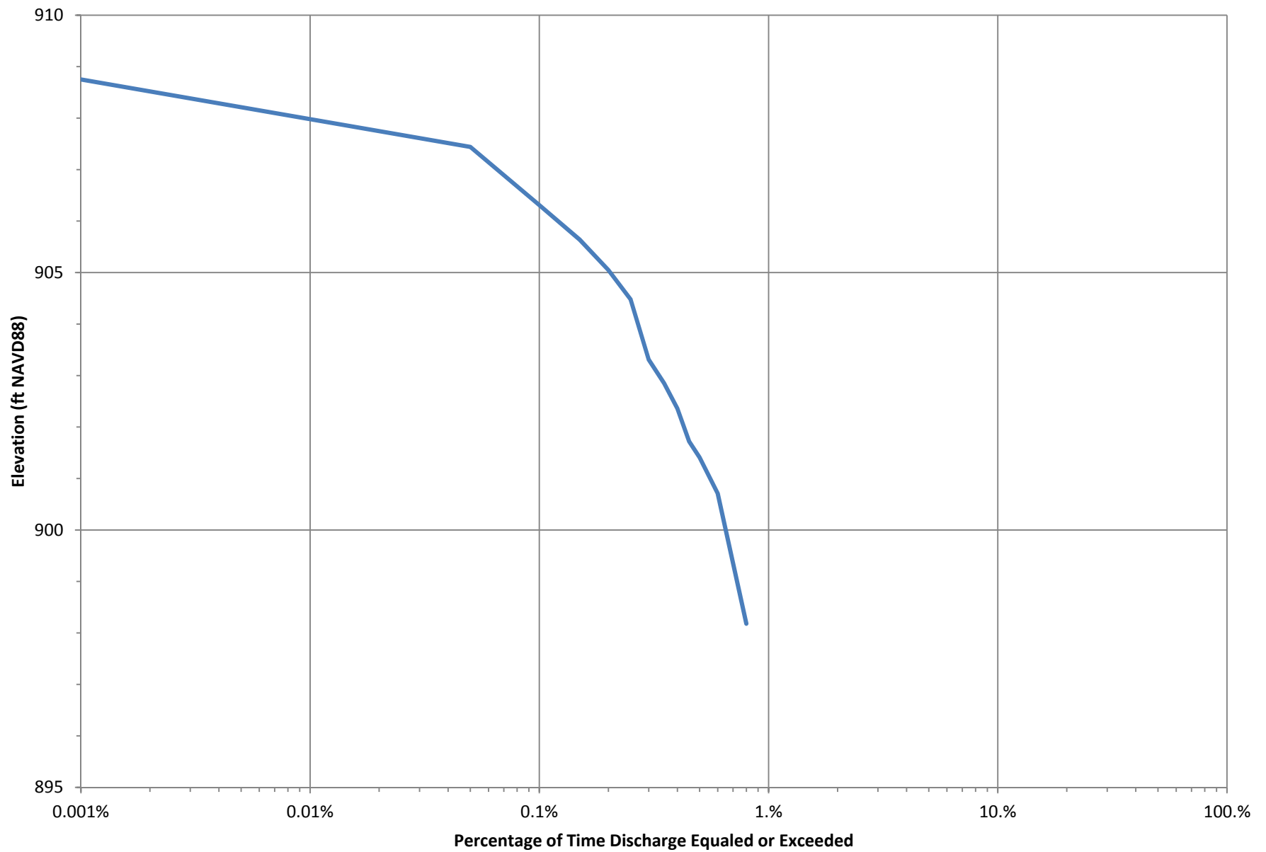
FCP Elevation-Duration Curve - FCP Alignment below Red River
