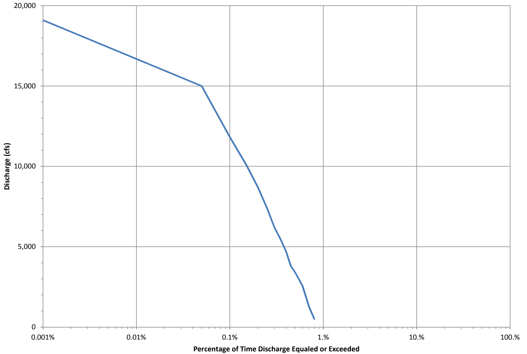
FCP Discharge-Duration Curve - FCP Alignment below Red River
